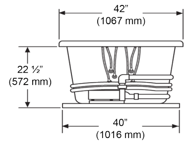
PLUMBING ROUGH-IN
