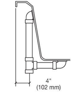
PLUMBING ROUGH-IN
