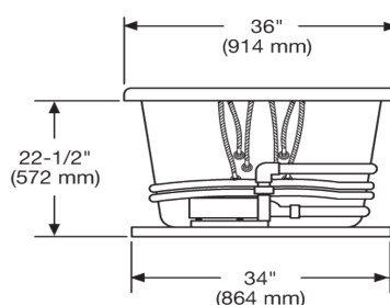
PLUMBING ROUGH-IN
