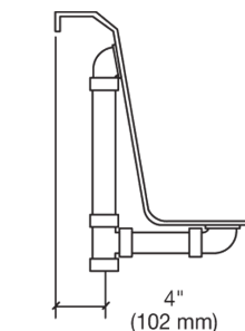
PLUMBING ROUGH-IN
