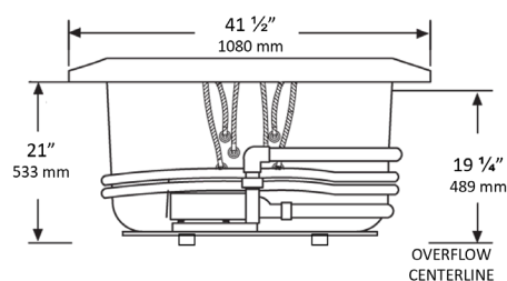
PLUMBING ROUGH-IN
