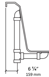
PLUMBING ROUGH-IN
