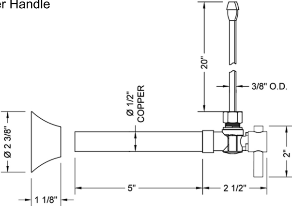
Contempo Lever Handle
