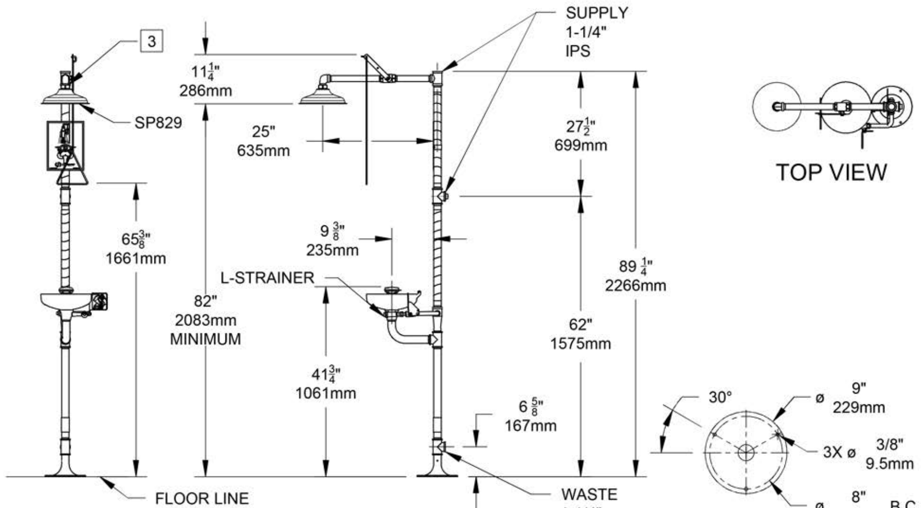
MOUNTING DETAIL SCALE 10:1
