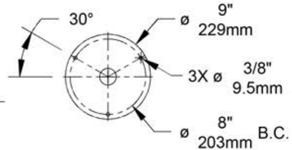
MOUNTING DETAIL SCALE 10:1
