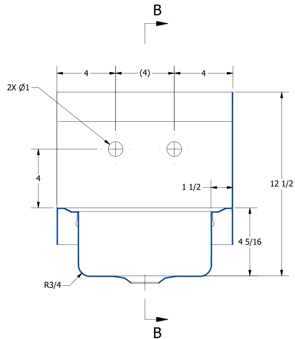
SECTION A-A SCALE 1 / 4
