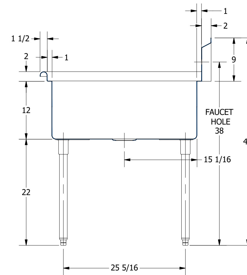
SECTION B-B SCALE 1:12
