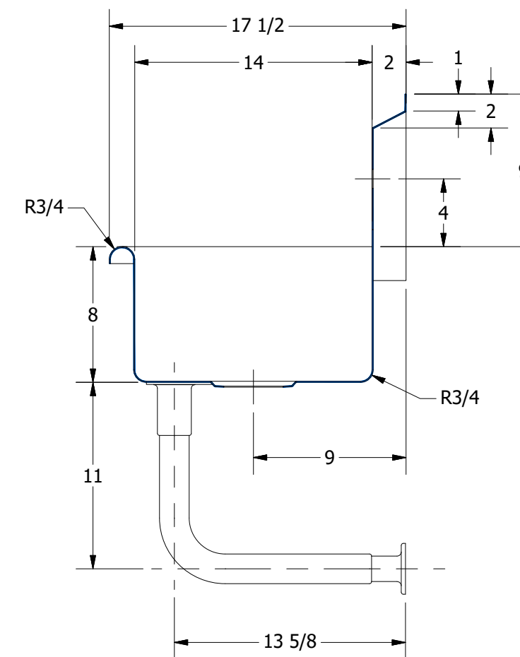
SECTION A-A SCALE 1/8
