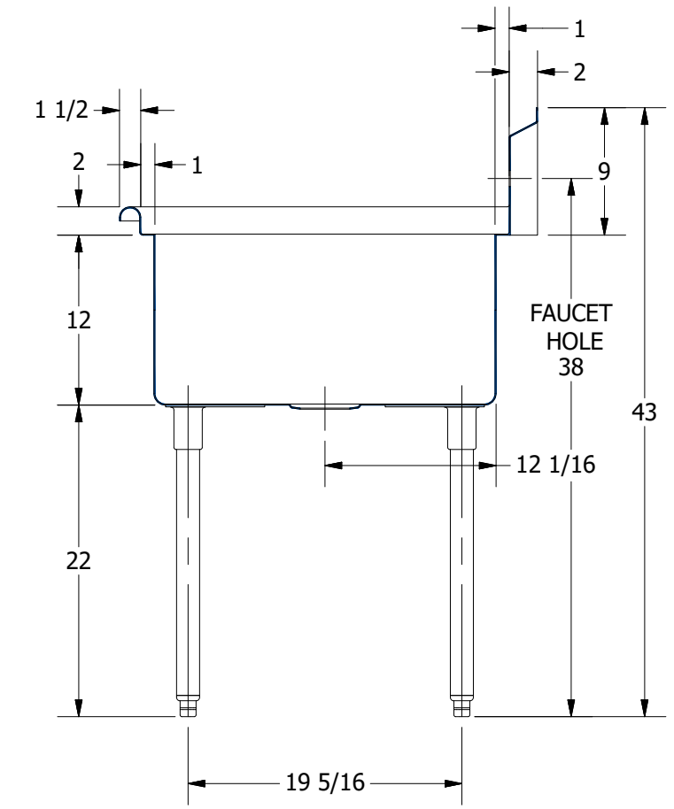
SECTION B-B SCALE 1:12
