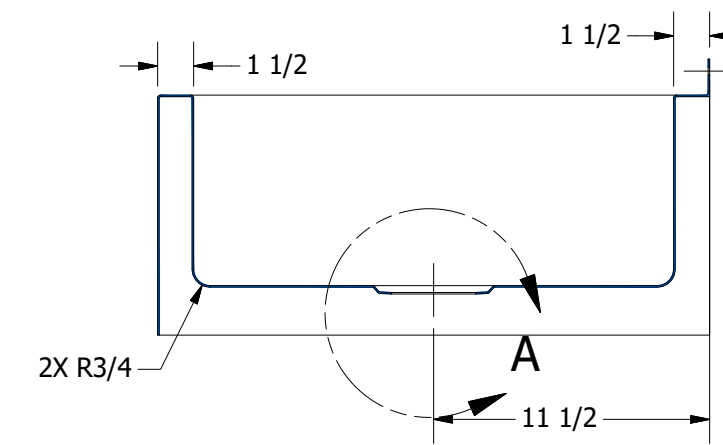
SECTION A-A SCALE 1/8
