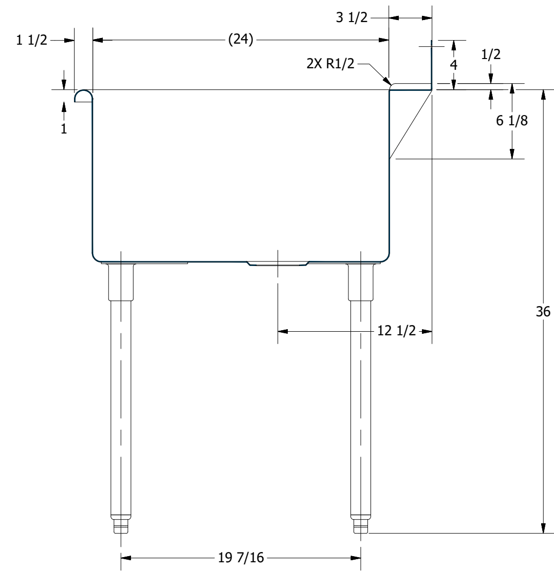
SECTION A-A SCALE 1/8
