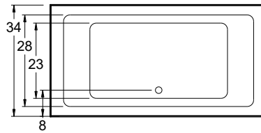
All bathtub dimensions are ± 1/2".
