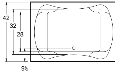
All bathtub dimensions are ± 1/2"
