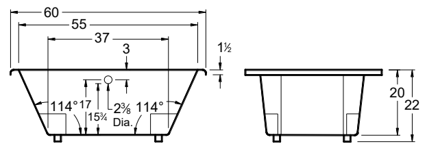
All bathtub dimensions are ± 1/2"
