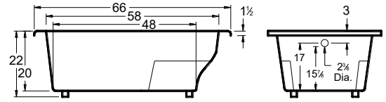
All bathtub dimensions are ± 1/2".
