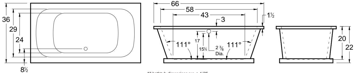
All bathtub dimensions are \pm 1/2" .
