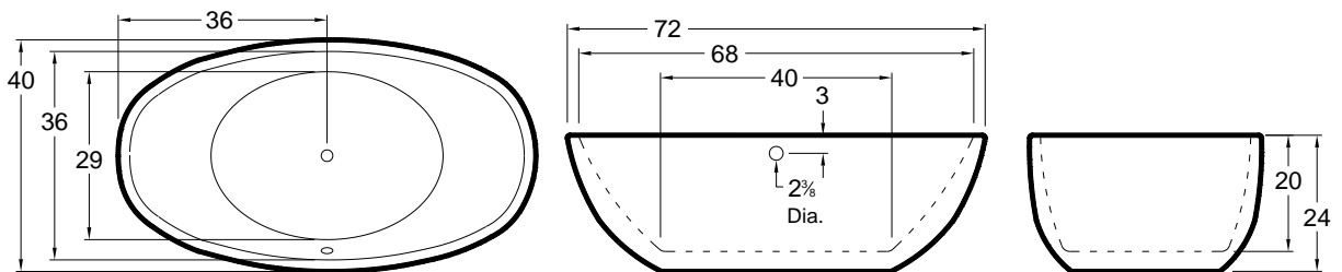
All bathtub dimensions are \pm 1/2 ".
